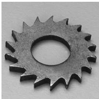
18 HOOKED TEETH (CHIPPER CUTTER)
